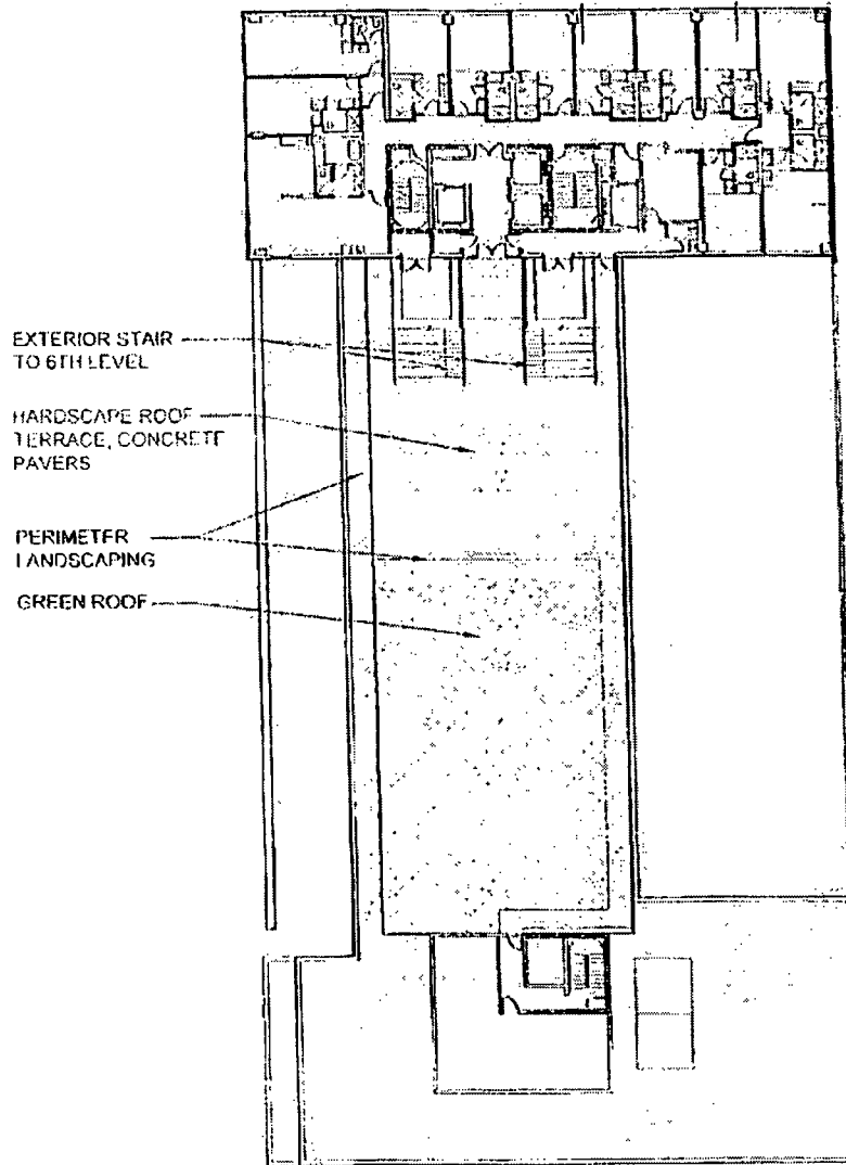
G. FIFTH LEVEL TERRACE LANDSCAPE PLAN SCALE: 1/32" = 1'-0"
