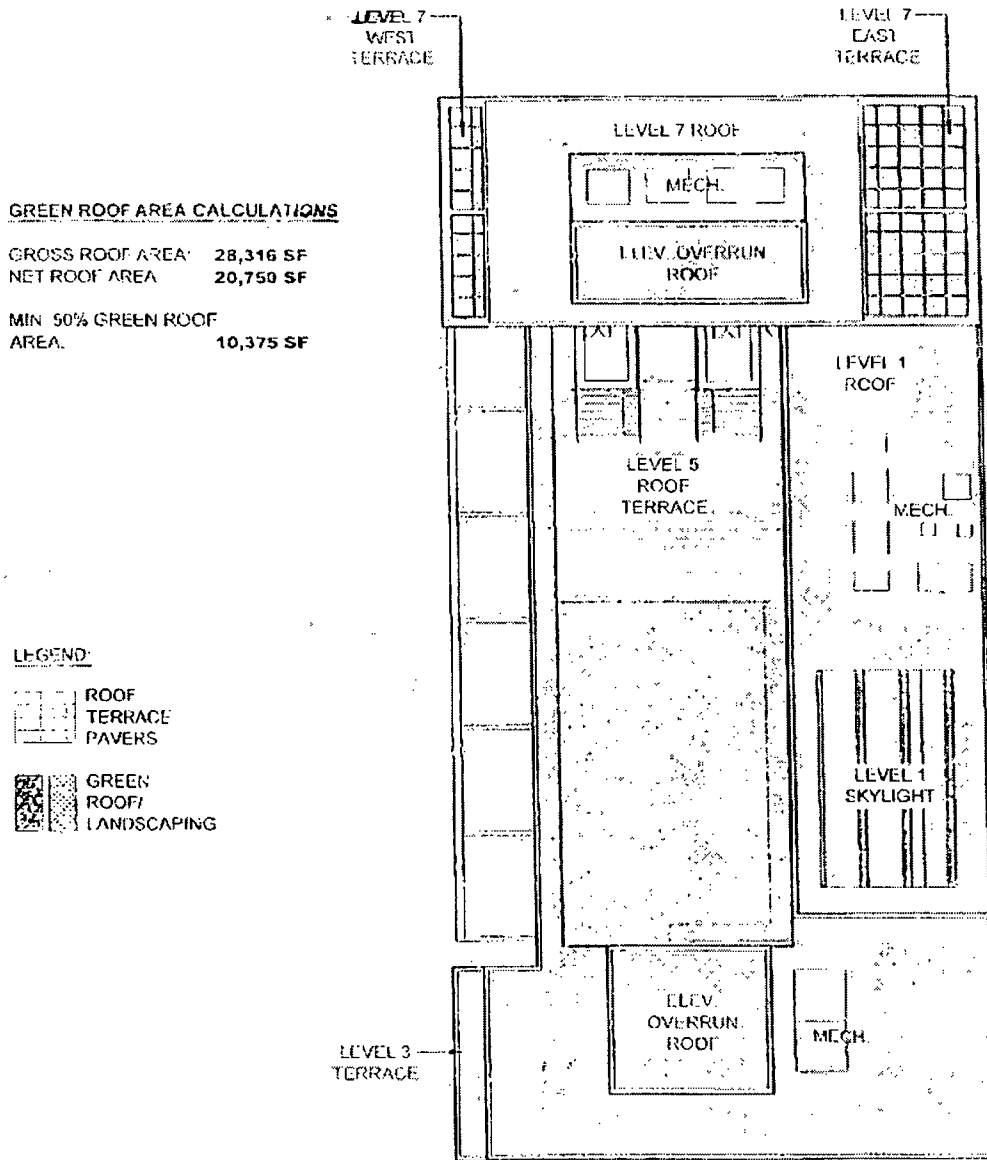
H. GREEN ROOF DIAGRAM SCALE 1/2" = 1'-0"
